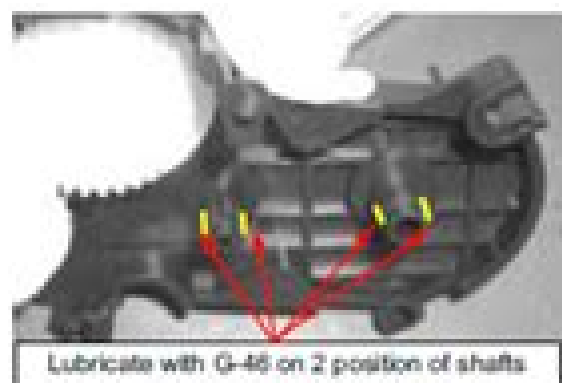
Figure 3-5. Lubrication point 2
