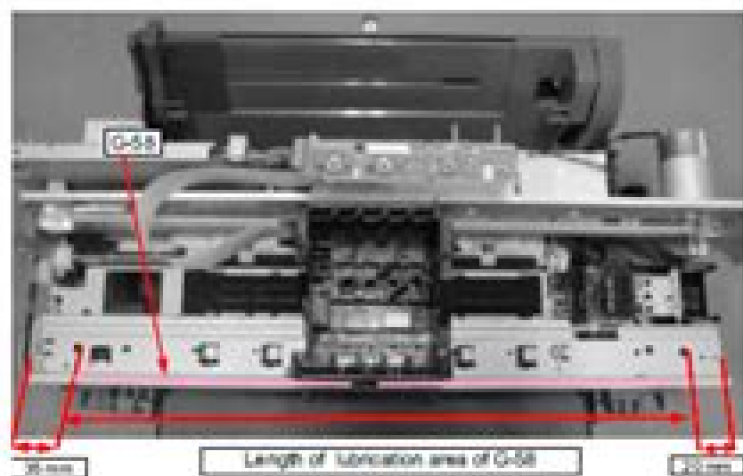
Figure 3-6. Lubrication point 3
