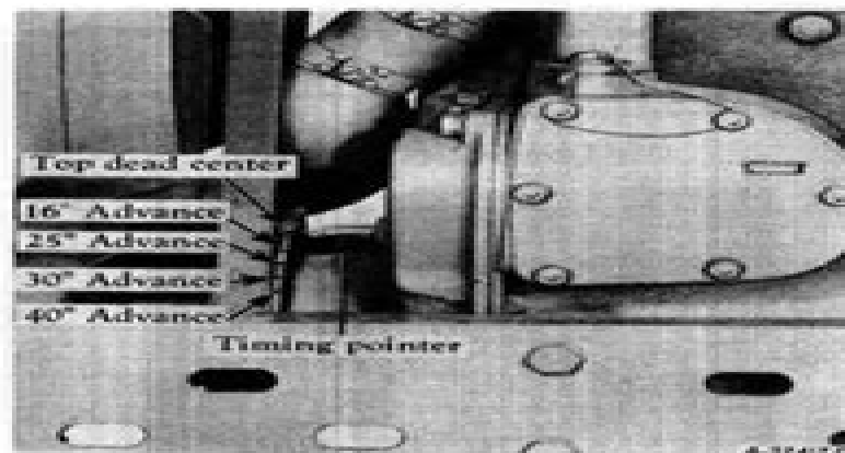
Illustr. 10 Timing pointer.
