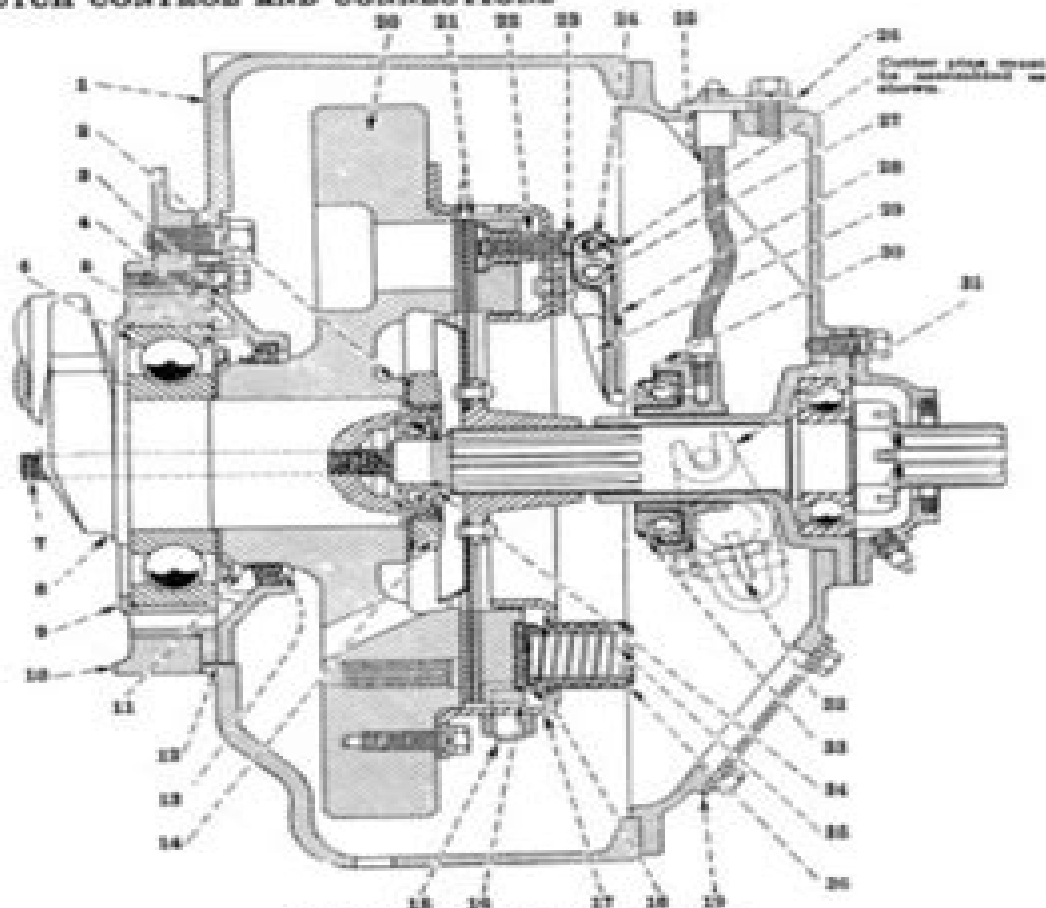
Clutch Control and Single Plate Clutch.
