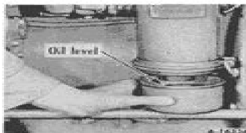
Illust. 27A Air cleaner oil cup.
