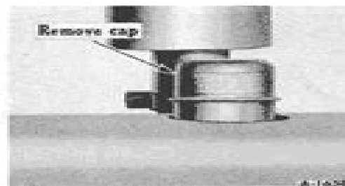
Illust. 27B Crankcase oil filler
