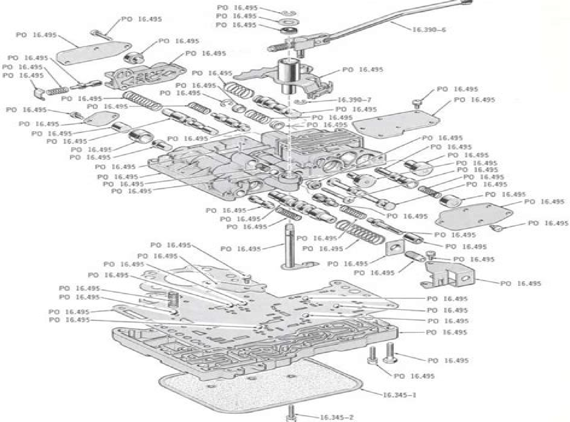
VALVE ASSEMBLY . . . 1972 (SIX-HEAVY DUTY)(V8)
